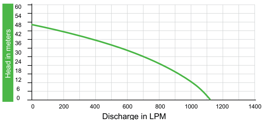
Performance Curve Dewatering submersible pump
