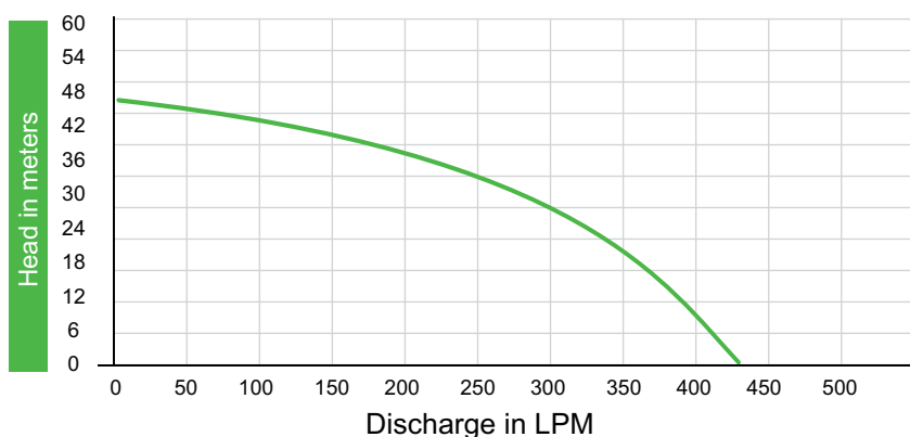
Performance Curve Dewatering submersible pump
