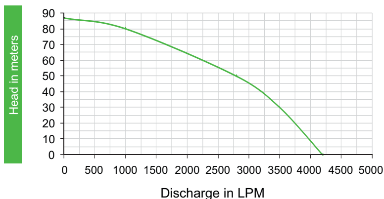
Performance Curve Dewatering Submersible Pump
