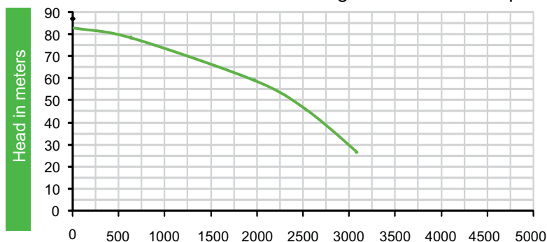
Performance Curve Dewatering Submersible Pump
