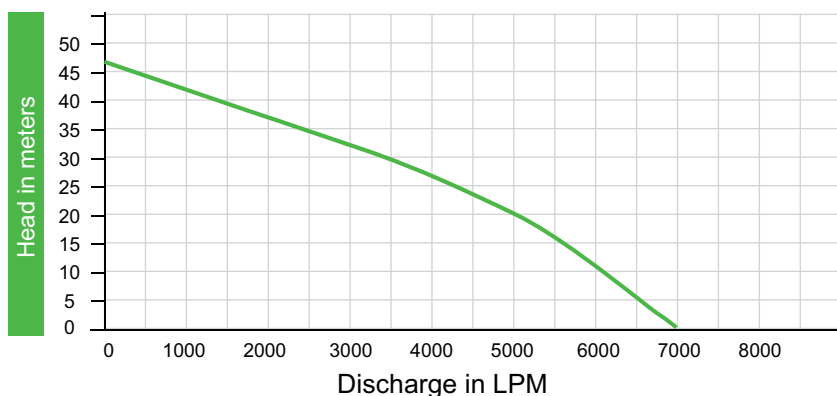
Performance Curve Dewatering submersible pump
