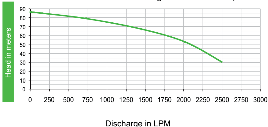
Performance Curve Dewatering Submersible Pump
