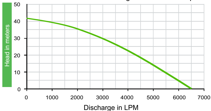
Performance Curve Dewatering Submersible Pump
