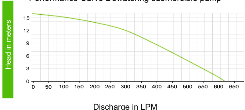
Performance Curve Dewatering submersible pump
