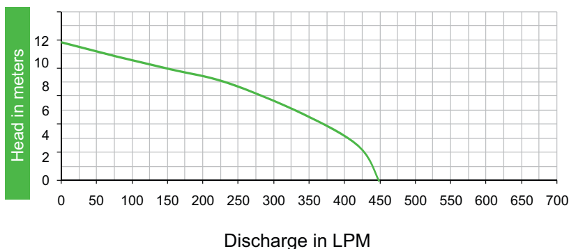
Performance Curve Dewatering Submersible Pump
